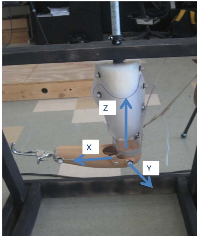
Figure 7 Coordinate system that defines the socket segment
